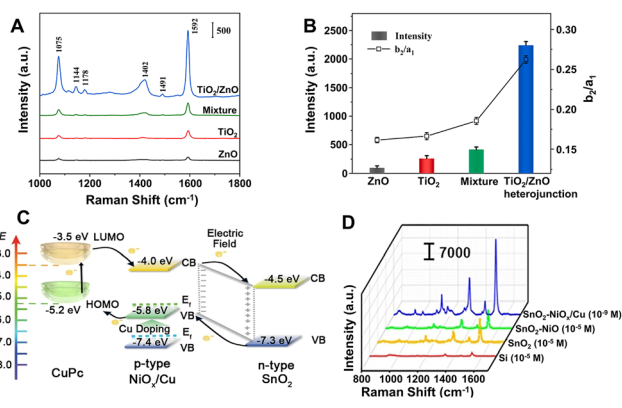
Fig. 12 (A) SERS spectra of 4-MBA ( 10^{-3} \text{ M} ) adsorbed on the surface of pure \text{TiO}_2 NPs, pure \text{ZnO} NPs, mixture of \text{TiO}_2 and \text{ZnO} NPs, and \text{TiO}_2/\text{ZnO} heterojunction composites. (B) The SERS intensity of the band at 1592 \text{ cm}^{-1} and the ratio of I_{1144}/I_{1075} ( I_{b2}/I_{a1} ) for different substrates. Reproduced from ref. 202 with permission from Elsevier, copyright 2022. (C) Energy level diagram of copper phthalocyanine (CuPc) molecule adsorbed on \text{SnO}_2\text{-NiO}_x/\text{Cu} SERS substrate. (D) Raman spectra of \text{SnO}_2\text{-NiO}_x/\text{Cu} ( 10^{-9} \text{ M} ), \text{SnO}_2 ( 10^{-5} \text{ M} ), \text{SnO}_2\text{-NiO} ( 10^{-5} \text{ M} ), and \text{SnO}_2 ( 10^{-5} \text{ M} ) substrates under 785 nm laser excitation. Reproduced from ref. 119 with permission from John Wiley & Sons, copyright 2021.
