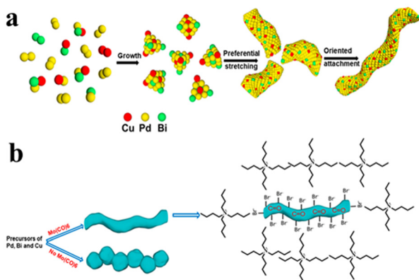
Fig. 10 Schematics illustrating the growth mechanism of PdBiCu nanowires, (a) morphology evolution of nanowires from the precursor nuclei, and (b) effect of Mo(CO) 6 presence on the morphology. Reprinted with permission from ref. 104. Copyright 2021 from the American Chemical Society.
