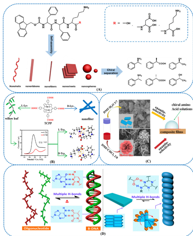
Fig. 5 (A) Schematic diagram of Fmoc-FFK, Fmoc-FFKK, and Fmoc-FFKD assemblies forming supramolecular nanostructures for chiral separation. 120 Reprinted from Y. Fan et al., Langmuir , 2020, 36 , 10361–10370 Copyright (2020), with permission from American Chemical Society. (B) Chiral enantioselective assemblies induced from achiral porphyrin by L- and D-Lysine. 133 Reprinted from S. Wu et al., Langmuir , 2019, 35 , 16761–16769 Copyright (2019), with permission from American Chemical Society. (C) Chiral flower-like and brick-like nanostructure films via solvent-tuned self-assembly and their enantioselective performances toward L-/D-amino acids. 134 Reprinted from K. Chen et al., Langmuir , 2019, 35 , 3337–3345 Copyright (2019), with permission from American Chemical Society. (D) Role of multiple hydrogen bonds in the induction and stabilization of a super-chiral B-DNA Structure; utilization of duplex hydrogen bonds among carboxylic acids and various pyridine-based binders to control the emergence of chiral nanostructures. 135 Reprinted from P. Xing et al., J. Am. Chem. Soc. , 2019, 141 , 9946–9954 Copyright (2019), with permission from American Chemical Society.
