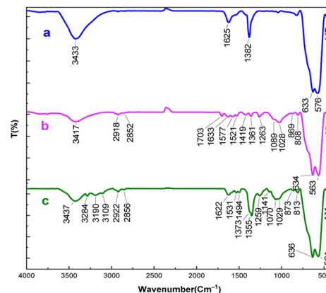
Fig. 1 FT-IR spectra of (a) \text{Fe}_3\text{O}_4 , (b) \text{Fe}_3\text{O}_4@\text{SiO}_2@\text{sil-acac} , (c) the [\text{Fe}_3\text{O}_4@\text{TAM-Schiff-base-Cu}^{(\text{III})}] complex.
