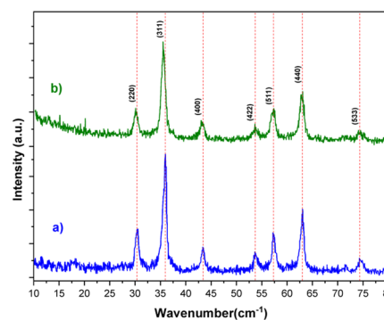
Fig. 2 XRD pattern of (a) \text{Fe}_3\text{O}_4 and (b) [\text{Fe}_3\text{O}_4@\text{TAM-Schiff-base-Cu}^{(\text{III})}] complex.
