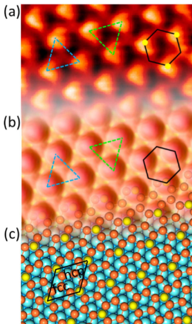
Fig. 7 Experimental (a) and simulated (b) STM images of the silicene/Ir(111) system. (c) Top view of the relaxed atomic model of the (\sqrt{3} \times \sqrt{3})/(\sqrt{7} \times \sqrt{7}) Ir(111) configuration. Adapted with permission from ref. 16, Copyright 2013 American Chemical Society.
