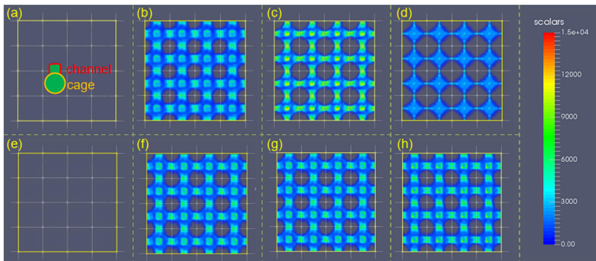
Fig. 9 The ethanol adsorption density distribution of W_s in l = 7.5 \text{ \AA} \times 4 \times 4 \times 4 supercell with fixed \epsilon = 2.52 \text{ kJ mol}^{-1} for (a) \sigma = 1 , (b) \sigma = 2 , (c) \sigma = 3 , and (d) \sigma = 4 \text{ \AA} . The ethanol adsorption density distribution of W_s in l = 7.5 \text{ \AA} \times 4 \times 4 \times 4 supercell with fixed \sigma = 2.2 \text{ \AA} for (e) \epsilon = 0.42 , (f) \epsilon = 1.68 , (g) \epsilon = 2.94 , and (h) \epsilon = 4.2 \text{ kJ mol}^{-1} .
