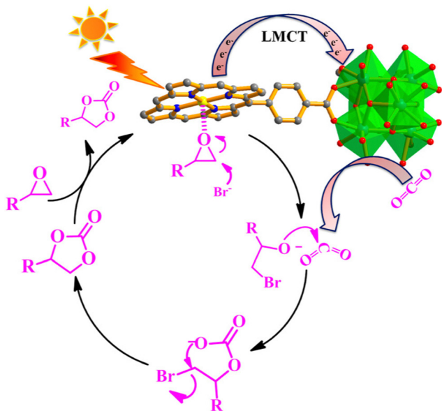
Fig. 22 Mechanism proposed for the PCN-224(Mg)-photocatalysed cycloaddition of epoxide to \text{CO}_2 . Reprinted with permission from ref. 239. Copyright 2022 American Chemical Society.
