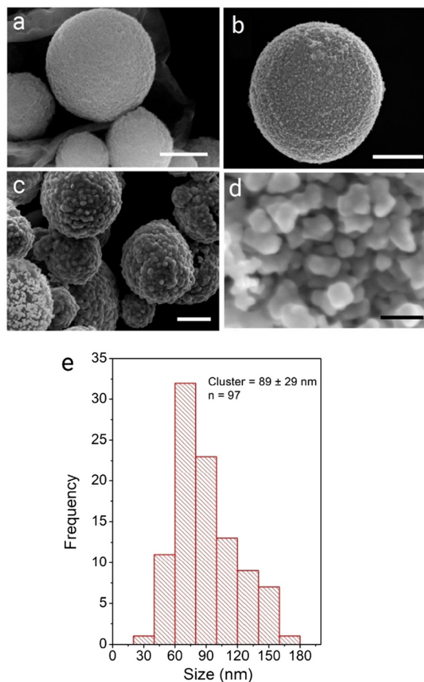
Fig. 1 SEM micrographs of precursor and composite systems prepared using approach 1: (a) o-C \mu P , (b) C \mu P-AuNP(DMAP) and (c and d) roughened composites C \mu P-AuNP-1 . Scale bars show (a–c) 500 nm and (d) 50 nm.
