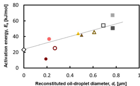
Fig. 13 Relationship between activation energy and reconstituted oil droplet diameters of the SQ powders. Powder prepared by homogenisation at \square , \bullet , \blacktriangle : 100 MPa, \triangle , \blacktriangle : 50 MPa and \square , \bullet , \blacktriangle : 20 MPa with 3 wt% NC is denoted by clear colour symbols, 5 wt% NC by light colour symbols, and 8 wt% NC by dark colour symbols. The rhombus key indicates the activation energy for the oxidation of the bulk oil of SQ. (Yoshii et al. , 2023) 46 "Reproduced from ref. 46 with permission from Taylor and Francis, copyright 2023".
