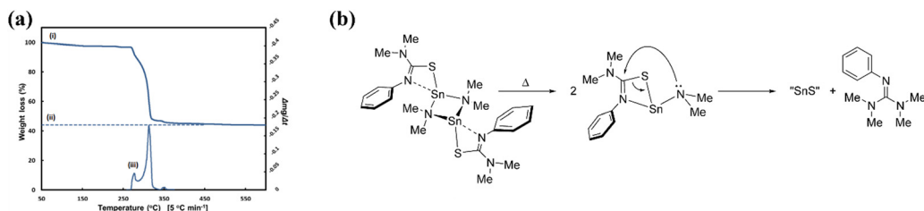
Fig. 27 (a) TGA of [\text{Sn}(\mu\text{-NMe}_2)(\text{SC}(\text{NMe}_2)\text{NC}_6\text{H}_5)]_2 , and the derivative of mass loss with respect to temperature to identify significant mass loss events, (b) suggested SnS formation mechanism from initial precursor. Reproduced with permission from ref. 242 copyright 2015, American Chemical Society.
