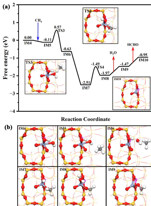
Fig. 5 The Gibbs free energy profile of the \text{HCHO} production branch over the \text{Cr}_1/\text{ZSM-5} SAC with the geometry structures of key transition states (a); the geometry structures of all the intermediates in the whole catalytic cycle (b). The Gibbs energy profile was calculated under the reaction conditions of 30 bar \text{CH}_4 , 0.5 M \text{H}_2\text{O}_2 at 323 K.
