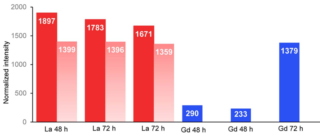
Fig. 3 Normalized intensity of La (red) and Gd (blue) measured in the total organisms and in the intestinal tract (light red) of the organisms. Beamline: NANOSCOPIUM. Incident energy of 17.02 keV.
