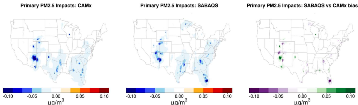
Fig. 3 Comparison of CAMx and 2023en-based SABAQS estimates of CPPP impacts on annual average primary PM_{2.5} (EC and crustal material). CAMx estimates shown on the left, SABAQS estimates shown in the middle and the difference between the two surfaces shown on the right with purple colors indicating a larger impact from SABAQS and green colors indicating a larger impact from CAMx.
