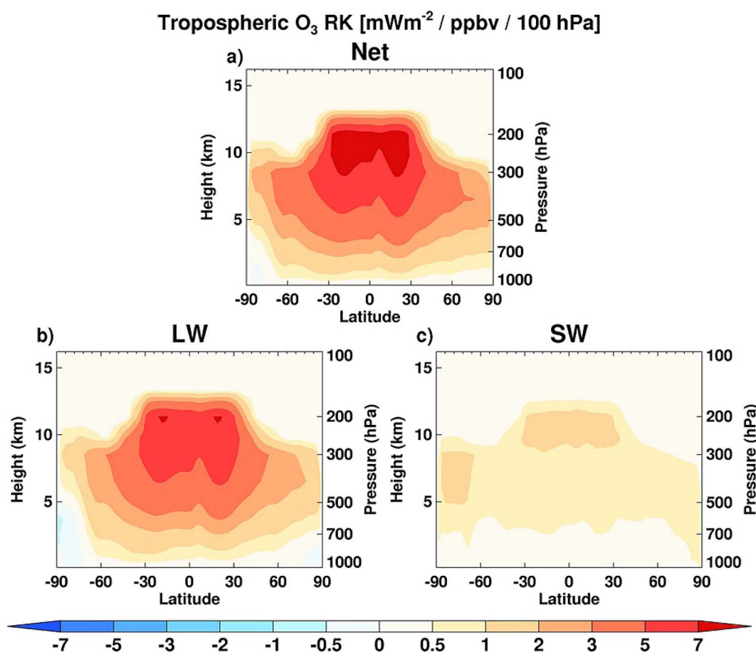
Fig. 11 Annual zonal mean tropospheric ozone radiative kernel (RK) 75 under all-sky conditions in units of \text{mW m}^{-2} \text{ppb}^{-1} / 100 \text{ hPa} for (a) net (LW + SW), (b) LW, and (c) SW. SW (short-wave) refers to the RF resulting from changes in the absorbed solar-radiation by the Earth-atmosphere system, which is mostly incident in the wavelength range 0.2 to 4 \mu\text{m} . LW (longwave) refers to changes in the outgoing longwave radiation at the top of the atmosphere; LW radiation (mostly in the wavelength range 4 to 400 \mu\text{m} sometimes) originates from emission by the Earth and its atmosphere and is modulated by absorption by atmospheric constituents. Radiative forcing is the sum of the individual SW and LW RFs. Note that this illustrates the general radiative response from tropospheric ozone, formed from precursor emissions of NO x , CO, CH 4 , HCs and is not an aviation perturbation. From Rap et al. (2015). 70
