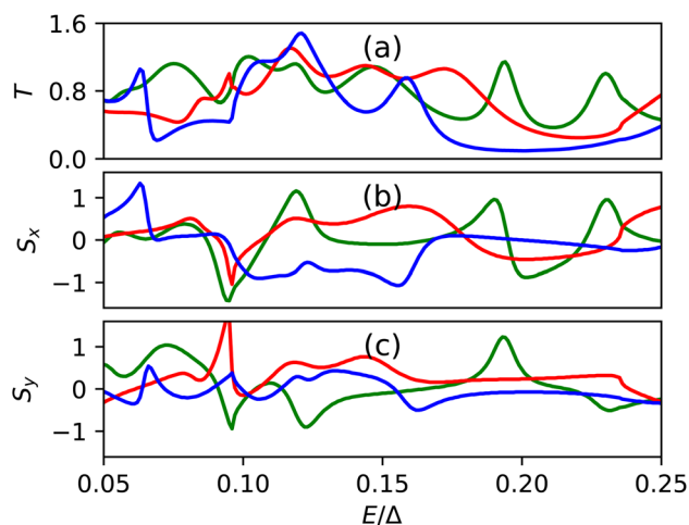
Fig. 3 Variation of (a) conductance ( T ) and the spin response, (b) S_x , and (c) S_y functions on the 6th magnetic site. Red, blue and green lines correspond three different magnetic configurations.
