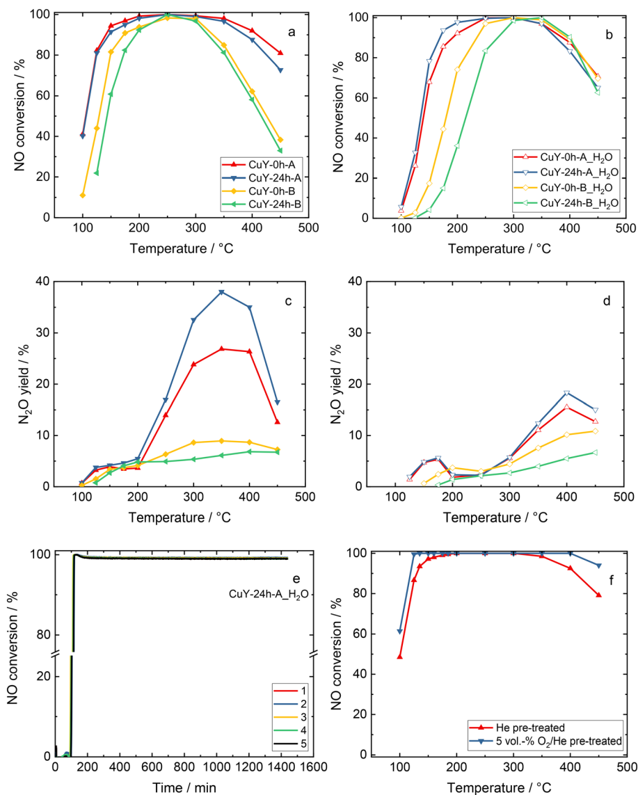
Fig. 10 a and b) NO conversion and c and d) \text{N}_2\text{O} yield during \text{NH}_3 -SCR-DeNO _x over copper-containing zeolite Y samples. Reaction conditions: m_K = 0.2 g; GHSV = 30\,000\text{ h}^{-1} ; c(\text{NO}) = 500 ppm, c(\text{NH}_3) = 575 ppm, c(\text{O}_2) = 4 vol%, ( c(\text{H}_2\text{O}) = 5 vol% when used), He balance, F_{\text{TOT}} = 120\text{ ml min}^{-1} , e) NO conversion over CuY-24h-A for five consecutive runs during the time-on-stream stability tests in the presence of water vapor at 200^\circ\text{C} , and f) NO conversion over CuY-24h-A after pre-treatment in He or 5 vol% \text{O}_2/\text{He} .
