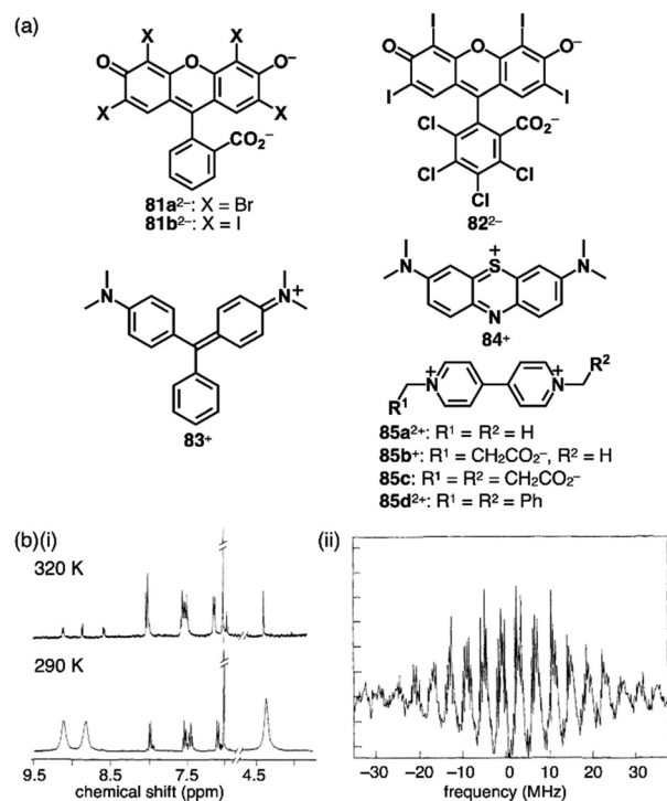
Fig. 42 (a) Xanthene-based \pi -electronic anions 81a , b 2− and the counteranions 83 , 84 + , 85a , d 2+ and 85b + and neutral 85c and (b) (i) 1 H NMR and (ii) ESR spectra of 85a 2+ – 81a 2− in DMSO- d 6 at 320 and 290 K and in DMSO at 295 K, respectively (redrawn from ref. 96c. Copyright 1992 ACS).
