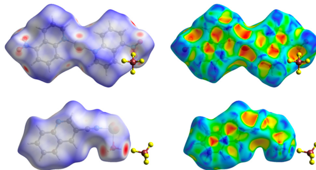
Fig. 9 Hirshfeld surfaces of complexes 1 (top) and 2 (bottom) excluding the BF 4 − counterion. From left to right mapped with the d -norm and shape index. Note that 2 is a polymer and therefore has significant spots around Ag from the propagation of the Ag–N and Ag–O bonds.
