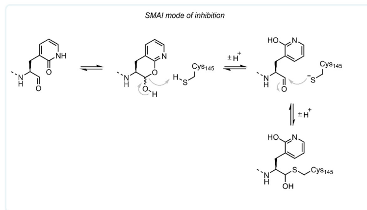
Scheme 2 Putative mechanism of reversible covalent inhibition of a cysteine protease by SMAls.
