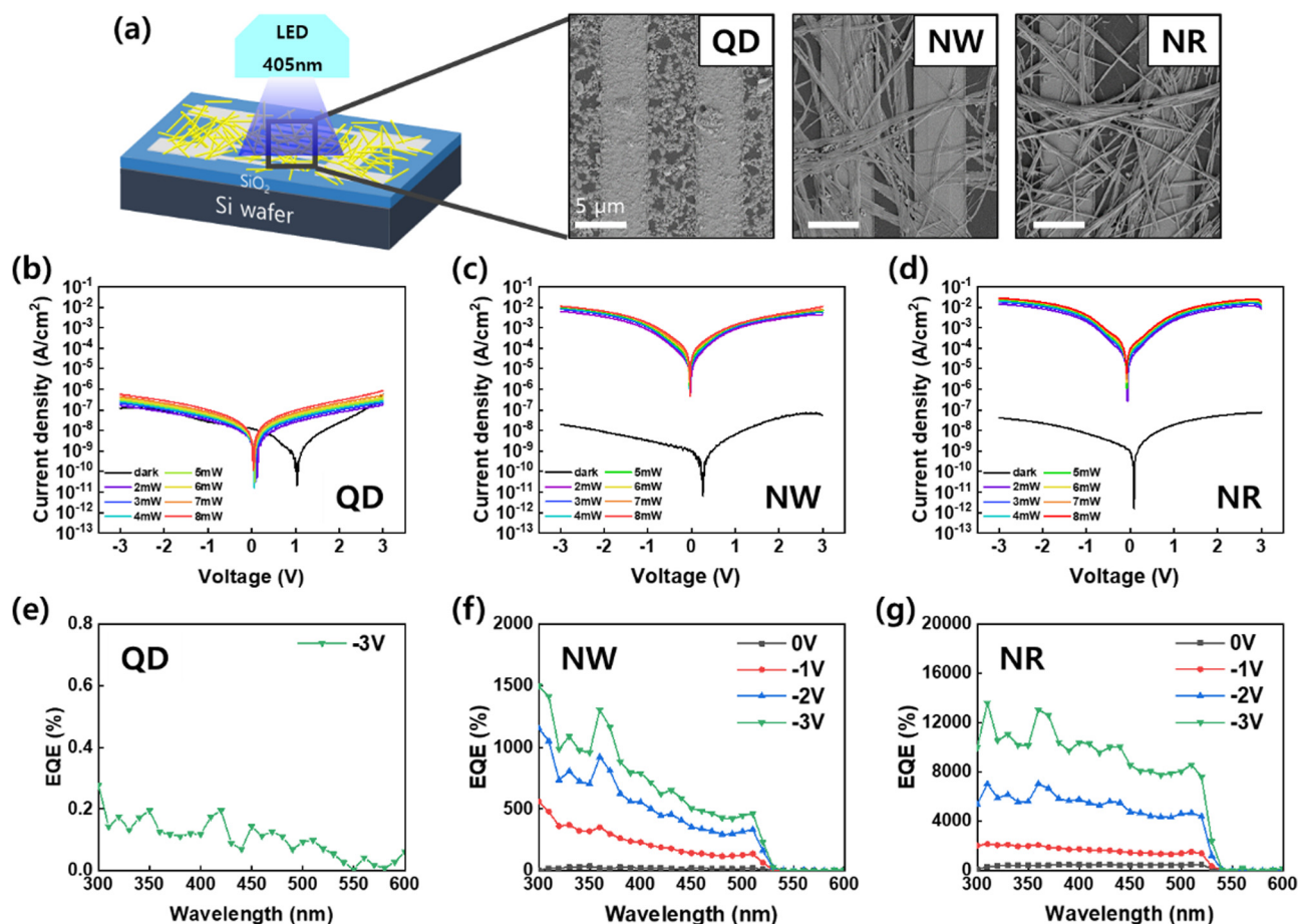
Fig. 5 (a) Schematic illustration of the constructed photodetector device and SEM images of the nanomaterials based on the \text{CsPbBr}_3 QDs, NWs, and NRs. J - V characteristics of the photodetectors under different illumination intensities based on the \text{CsPbBr}_3 (b) QDs, (c) NWs, and (d) NRs. EQE spectra of the photodetectors at various bias voltages based on the \text{CsPbBr}_3 (e) QDs, (f) NWs, and (g) NRs.
