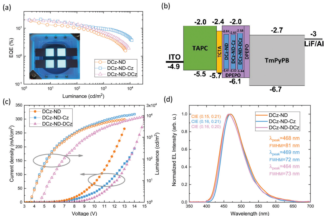
Fig. 5 Main characteristics of naphthyrindine-based TADF-OLEDs: (a) EQE vs. luminance with a picture of a working DCz-ND-Cz device in the inset; (b) energy level diagram; (c) current density and luminance vs. applied voltage; and (d) EL spectra at 100 cd m -2 .
