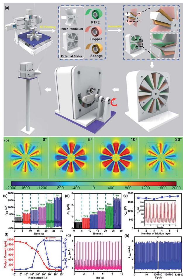
Fig. 2 (a) The schematic structure and fabrication process of the PMLA-TENG. (b) The potential distributions of different angles simulated by COMSOL. Functional parameters (c) I_{SC} , (d) Q_p , and (e) V_{OC} of the PMLA-TENG with different pairs of friction layers. (f) The relationship between the loading resistance, instantaneous current and power density of the TENG with six friction layers. (g) I_{SC} after processing by a transformer and a rectifier. (h) The I_{SC} processed by a transformer and a rectifier after about 136 800 cycles (working continuously for 6 h). Reproduced with permission. 59 Copyright 2019, Elsevier.
