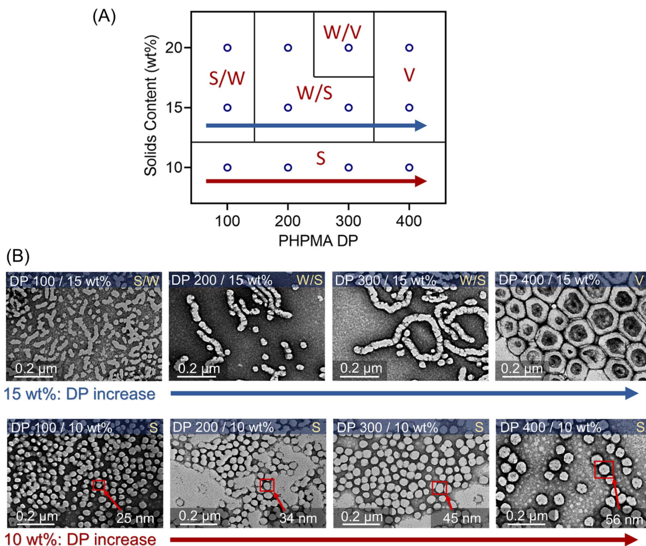
Fig. 6 (A) Phase diagram of photo-PISA synthesized by ZnPcS 4 - mediated dispersion photopolymerization of HPMA. Polymerizations were conducted under the irradiation of 730 nm light ( I = 60 \text{ mW cm}^{-2} ) for 24 hours without prior deoxygenation in water at fixed reaction stoichiometries of [PEG 113 -CDTPA] : [TEOA] : [ZnPcS 4 - ] 1 : 4 : 0.02. (B) TEM images of synthesized polymeric nanoparticles at 10 and 15 wt% solids content (note: TEM images at 20 wt% were presented in Fig. 5C).
