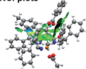
Scheme 26 Cu-catalyzed radical asymmetric synthesis of allenes from 1,3-enynes and, the optimized structures and NCI plots of TS-L4-R1 and TS-L4-S1. The dihedral angle between planes of the aromatic substituent (pink plane) and the oxazoline (cyan plane) is denoted as \phi .
