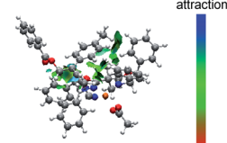
Scheme 26 Cu-catalyzed radical asymmetric synthesis of allenes from 1,3-enynes and, the optimized structures and NCI plots of TS-L4-R1 and TS-L4-S1. The dihedral angle between planes of the aromatic substituent (pink plane) and the oxazoline (cyan plane) is denoted as \phi .
