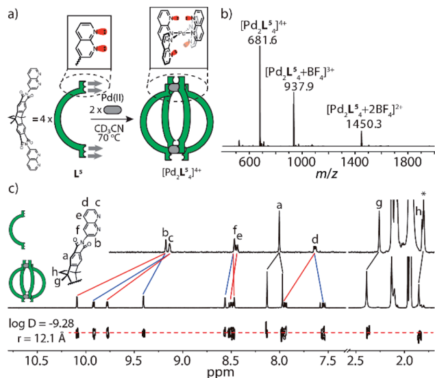
Fig. 2 (a) Self-assembly and characterization of homoleptic cage [\text{Pd}_2\text{L}_5]_4 with trans - [\text{Pd}(\text{up-}\text{L}^{\text{Na}})_2(\text{down-}\text{L}^{\text{Na}})_2] ligand arrangement around both coordination sites; (b) high resolution ESI mass spectrum of [\text{Pd}_2\text{L}_5]_4^{4+} and \text{BF}_4^- adducts; (c) ^1\text{H} NMR spectra (600 MHz, 298 K, \text{CD}_3\text{CN} ) of ligand \text{L}^5 (top), cage [\text{Pd}_2\text{L}_5]_4 (middle, 0.64 mM) and its DOSY trace (bottom).
