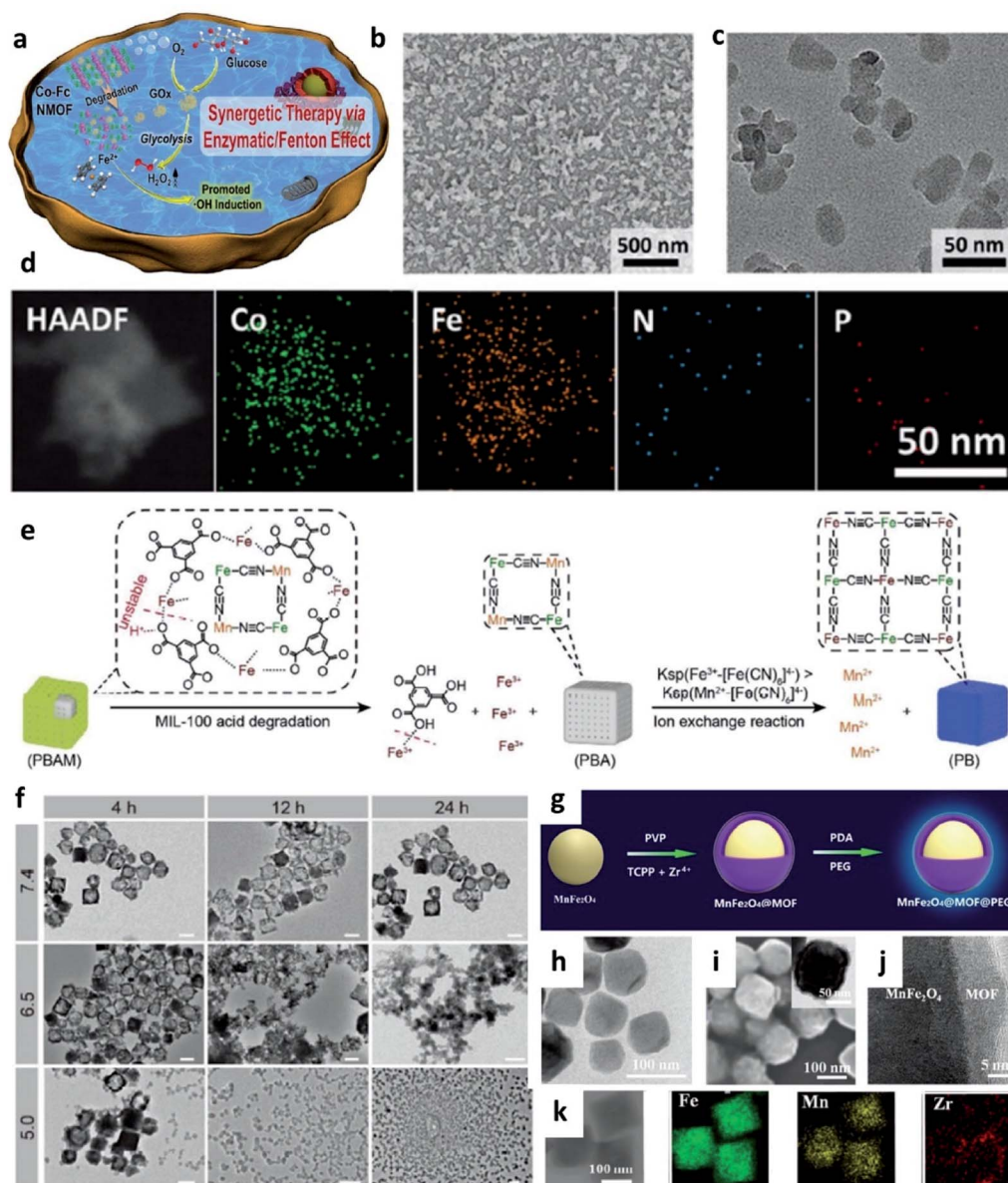
Fig. 8 (a) Schematic synthetic process of Co-Fc@GOx (nanoscale Co-ferrocene metal–organic framework, Co-Fc NMOF) as a cascade Fenton and enzymatic reaction nanoplatform for promoted • OH generation. (b–d) SEM, TEM image, and elemental mapping image of Co-Fc@GOx NMOF. Reproduced with permission from ref. 51. Copyright 2020, Wiley-VCH. (e) Schematic illustration of acid degradation and the rapid ion exchange reaction during the nanotheranostic agents (NTAs) synthesis process. K_{sp} : stability constant. (f) TEM images of PBAM (a MIL-100 (Fe)-coated Prussian blue (PB) analogue ( K_2\text{Mn}[\text{Fe}(\text{CN})_6] )) in different pH conditions (pH = 5.0, 6.5, and 7.4). Scar bar: 100 nm. Reproduced with permission from ref. 52. Copyright 2020, Wiley-VCH. (g) Schematic synthetic process of MnFe 2 O 4 @MOF. (h) TEM image of MnFe 2 O 4 NP. (i) SEM, TEM (inset), (j) high-resolution TEM, and (k) elemental mapping images of MnFe 2 O 4 @MOF. Reproduced with permission from ref. 53. Copyright 2019, Wiley-VCH.
