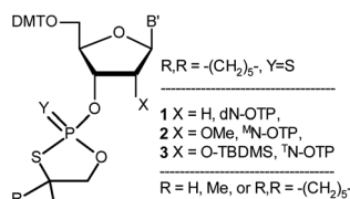
Chart 1 Classes of the OTP derivatives of 2'-deoxyribo- and ribonucleosides. \text{B}' = \text{Ade}^{\text{Bz}} , \text{Cyt}^{\text{Bz}} , \text{Gua}^{\text{IBu}} , or Ura. For those with \text{R} = \text{H} or Me, see ref. 13 and 16, respectively.
