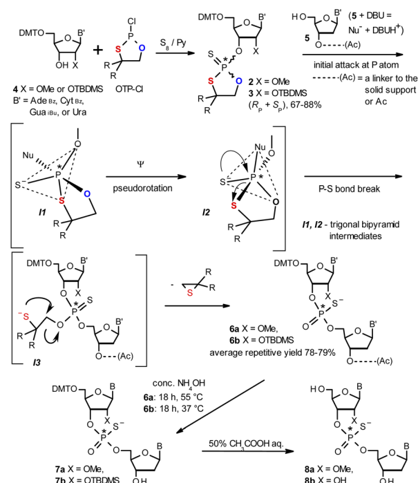
Scheme 1 Synthesis of OTP monomers 2 and 3 ( \text{R, R}' = -(\text{CH}_2)_5- ) and the mechanistic principle of the coupling step.
