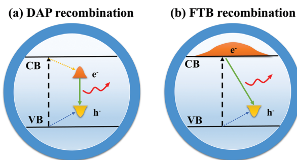
Fig. 7 Schematic representation of the (a) DAP recombination and (b) FTB recombination.
