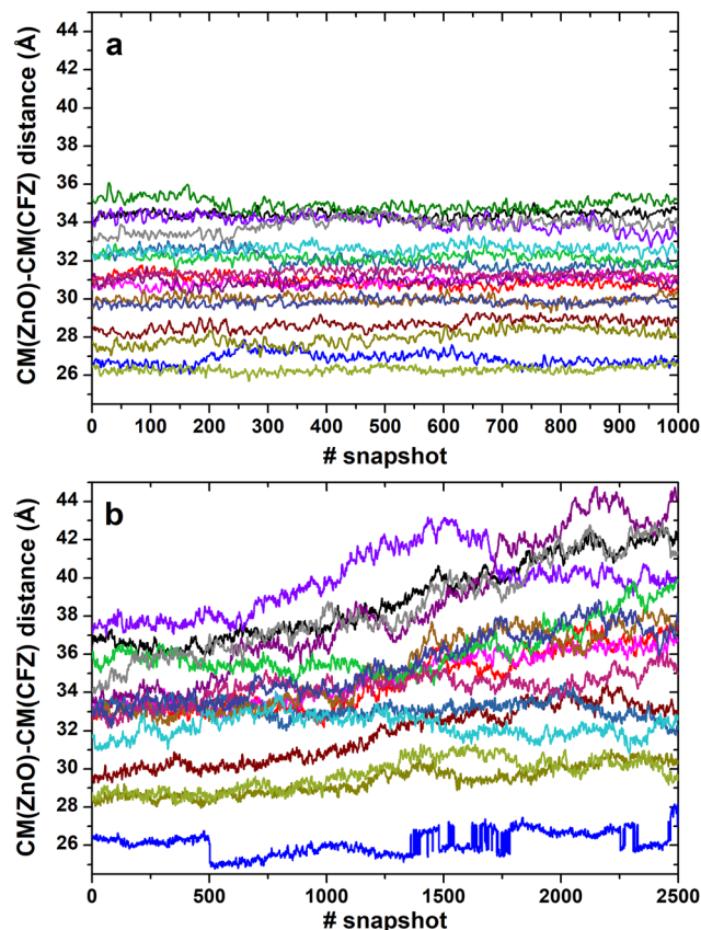
Fig. 8 Evolution of the distance between the center of mass of the ZnNP and the center of mass of each adsorbed CFZ molecule (represented by the various color lines) in ethanol (last 200 ps) (a) and water (last 500 ps) (b) solutions.
