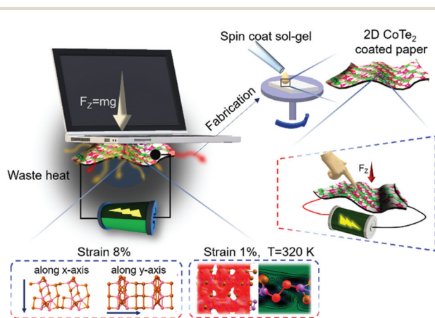
Fig. 1 Schematic representation of the utilization of waste heat by generating electricity and the energy harvesting concept of piezo-tribo generators using 2D \text{CoTe}_2 .
