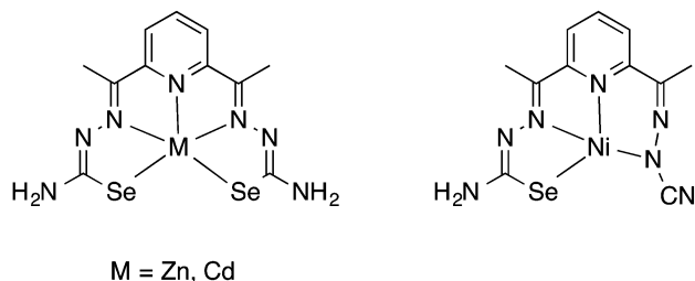
Fig. 16 Examples of complexes with multidentate selenosemicarbazone ligands.
