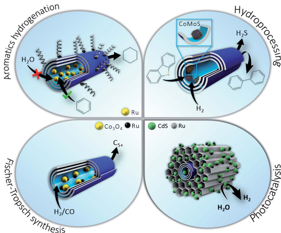
Scheme 5 Nanoreactors templated on clay nanotubes for catalytic hydrogenation of aromatics in water media, dibenzothiophene hydrodesulfurization, and Fischer–Tropsch synthesis and photocatalysis.
