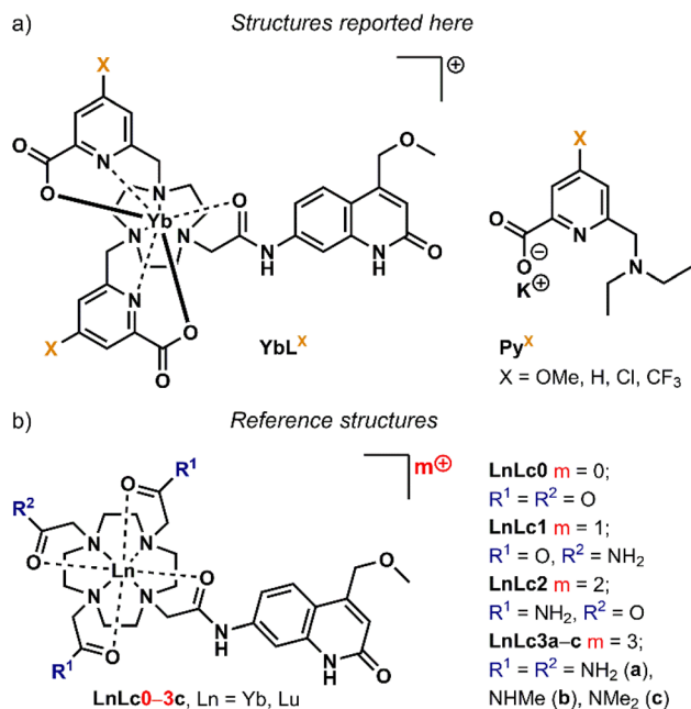
Fig. 2 (a) Complexes studied here (YbL X ) and pyridine model compounds (Py X ), X is the pyridine p -substituent. (b) Cyclen-based Yb complexes used as the reference structures (YbLc), LnLc0–3c are cyclen-based complexes with 0 to +3 overall charge.
