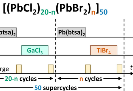
Fig. 9 Scheme of a pulse sequence used to deposit mixed lead halides. \text{PbCl}_2 and \text{PbBr}_2 binary processes are used as an example. The total number of deposition cycles was always 1000, as n \leq 20 .
