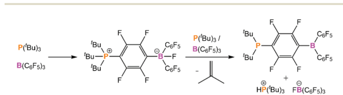
Scheme 2 Possible side-reaction between P(tBu)_3 and B(C_6F_5)_3 .
