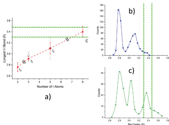
Fig. 10 Informed assignment of the I_{11}-I_{10}-I_9 \cdots I_8-I_7 \cdots I_6-I_5-I_4 complex. Green dashed lines represent dotted interactions in the formula. (a) Graphical representation of Table 1 data, i.e. , average value \pm FWHM of the longest bond length in examined polyiodides (black slashes signal different polyiodide charges). Superposition of distances under discussion with pentaiodide (b) and octaiodide (c) bond length distributions. While possible, an I_5^- \cdots I_3^- assignment would require both a quite unusual I_5^- bond length (on the fringe of the Gaussian) and a short non-explained I_5^- \cdots I_3^- contact. Assignment to distorted I_8^{2-} instead makes both distances close to statistical maximum, one shorter and one longer as expected in the case of distortion, a very common phenomenon in polyiodides.
