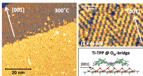
Fig. 13 Left: Large scale image of 1 ML obtained upon thermal desorption at 300^\circ\text{C} of a bi-layer of 2H-TTP deposited at RT (+2.5V, 100 pA); all terraces are covered with an extended (2 \times 4) -obl phase, entirely composed of metalated TPP molecules. Right: A smaller scale image of the same film puts in evidence the saddle-shape of the metalated molecules, and a small asymmetry with respect to the major axis due to the small azimuthal rotation of the molecules in the ordered phase, as compared to the isolated ones. Inset panel: A side-view of the equilibrium configuration of an isolated \text{TiO}_2^{\text{br}}\text{-TTP} molecules puts in evidence the bonding of molecular Ti with the two O_{\text{br}} atoms underneath.
