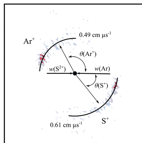
Fig. 1 CM scattering diagram for the reaction S^{2+} + Ar \rightarrow S^{+} + Ar^{+} at a CM collision energy of 5.3 eV. The black dot indicates the position of the CM. The intensity scale is logarithmic. See text for details.
