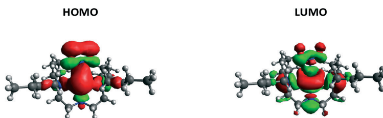
Fig. 8 Calculated frontier molecular orbitals for (a) 1 (polymorph II) and two other Pd(II)–nitrite molecules reported in the literature, capable of 100% conversion to a nitrito-( \eta^1 -ONO) excited state: (b) [Pd(Et 4 dien)(NO 2 )] + , 37 and (c) [Pd(Bu 4 dien)(NO 2 )] + . 38
