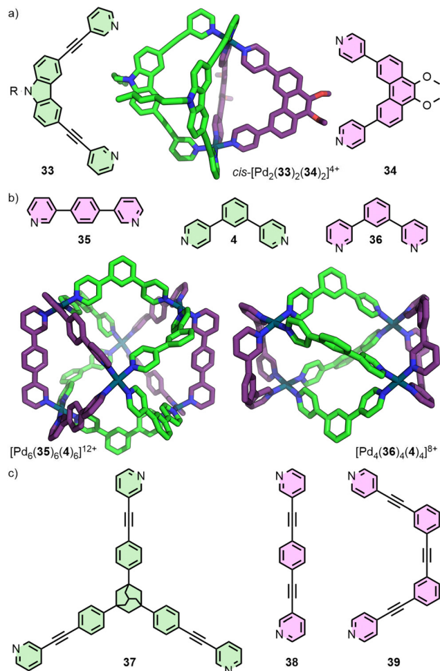
Fig. 8 (a) Geometric complementarity between ditopic ligands 33 and 34 facilitates access to the heteroleptic cage \text{cis-}[\text{Pd}_2(\mathbf{33})_2(\mathbf{34})_2]^{4+} (SCXRD structure). (b) Higher nuclearity heteroleptic structures have also been reported, such as [\text{Pd}_6(\mathbf{35})_6(\mathbf{4})_6]^{12+} and [\text{Pd}_4(\mathbf{36})_4(\mathbf{4})_4]^{8+} (SCXRD structures). (c) Through matching of ligand geometries, in combination with denticity mismatch, trigonal prismatic cages [\text{Pd}_3(\mathbf{37})_2(\mathbf{38}/\mathbf{39})_3]^{6+} have been realised.
