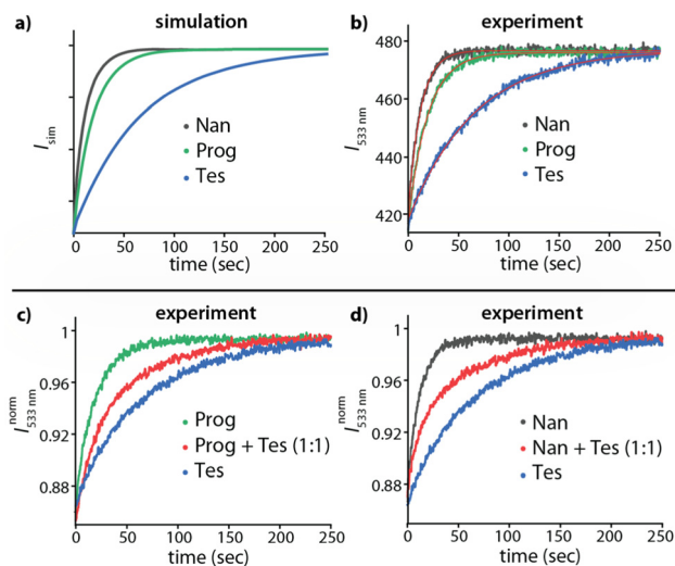
Fig. 4 (a) Simulated kinADA and (b) Experimental kinADA PFO traces monitored at 533 nm ( \lambda_{\text{exc}} = 376 nm) for \text{CB8} \rightarrow \text{Tes} (1 \mu\text{M} , blue), \text{CB8} \rightarrow \text{Prog} (1 \mu\text{M} , green) and \text{CB8} \rightarrow \text{Nan} (1 \mu\text{M} , black) host \rightarrow analyte complex upon spiked addition of MPCP dye (50 \mu\text{M} ) in water. See Fig. S5 and S6 in the ESI† for further details and parameters used for the simulation. The red line in Fig. 4b depicts the fitted data according to the kinADA PFO binding model (eqn (1)). Experimental kinADA PFO traces monitored at 533 nm ( \lambda_{\text{exc}} = 376 nm) for a mixture of two steroids as analytes (red curve) in case of (c) \text{CB8} (1 \mu\text{M} ), \text{Tes} (0.5 \mu\text{M} ) and \text{Prog} (0.5 \mu\text{M} ) and (d) \text{CB8} (1 \mu\text{M} ), \text{Tes} (0.5 \mu\text{M} ) and \text{Nan} (0.5 \mu\text{M} ) upon spiked addition of MPCP (50 \mu\text{M} ) in water. The kinetic traces for individual steroids are shown for comparison.
