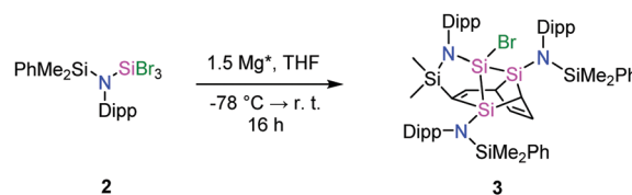
Scheme 1 Reductive debromination of the tribromoamidosilane 2 to the silaheterocycle 3 ( Dipp = 2,6\text{-}^iPr_2C_6H_3 ).
