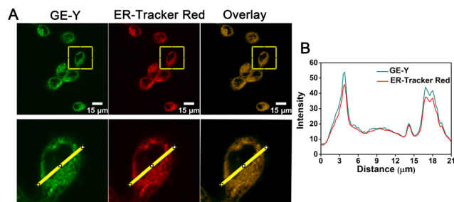
Fig. 2 (A) Colocalization cell images of GE-Y . MCF-7 cells co-stained with 10 \mu\text{M} GE-Y and 1 \mu\text{M} ER-Tracker Red for 20 min. Green channel ( \lambda_{\text{ex}} = 488 nm, \lambda_{\text{em}} = 520–560 nm, voltage of PMT: 550 V): GE-Y . Red channel ( \lambda_{\text{ex}} = 561 nm, \lambda_{\text{em}} = 600–640 nm): ER-tracker Red. Top row: The whole images; bottom row: enlarged regions of interest (ROI) of the top row. Scale bar is 15 \mu\text{m} . (B) ImageJ software was used for the fluorescence intensity profile of bottom row ROI analysis. The red line was from ER-Tracker Red, and the green line was from GE-Y .
