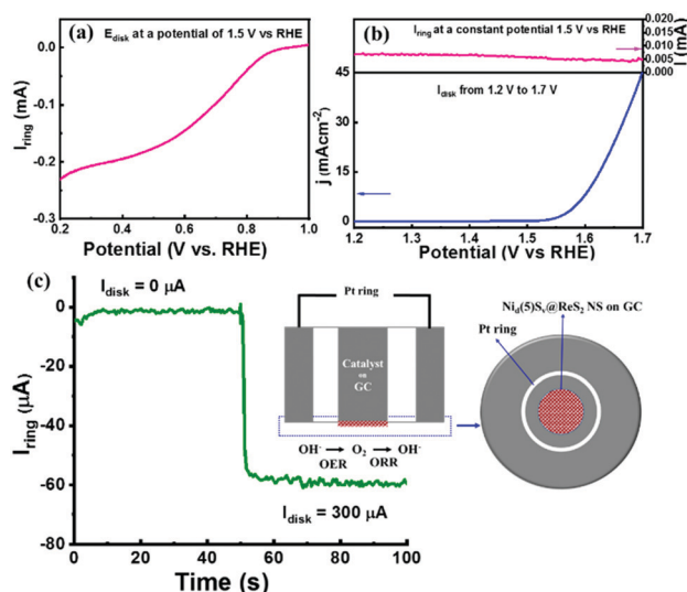
Fig. 4 (a) RRDE LSV plot of \text{Ni}_d(5)\text{S}_v\text{@ReS}_2 NS showing the ORR on the ring electrode at a disk potential of 1.5 V (vs. RHE), (b) OER LSV plot on the disk electrode measuring the current response on the ring electrode and (c) faradaic efficiency (FE) calculation using the RRDE techniques (inset shows the FE testing mechanism and RRDE configuration).
