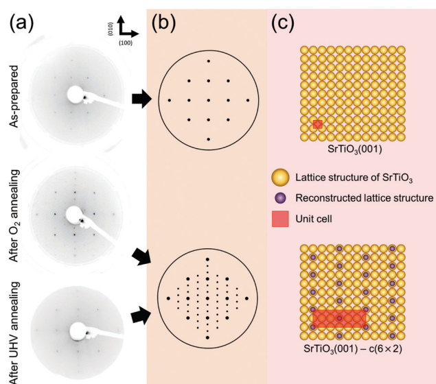
Fig. 2 (a) LEED patterns of the as-prepared, O 2 annealed and UHV annealed SrTiO 3 (001) surface at 600 °C. (b) Simulated LEED patterns for structural analysis. (c) The illustrations of lattice structures in real space.
