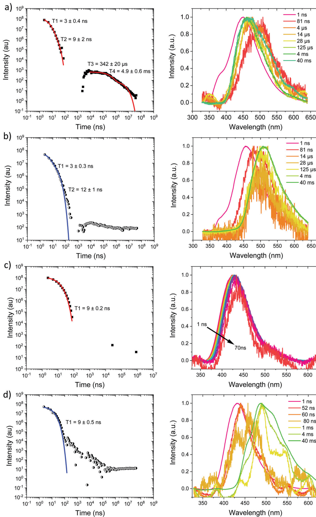
Fig. 5 Time-resolved spectroscopically integrated intensity decay (left) and representative time resolved spectra (right) of (a) \text{Ph}_2\text{TRZCzPhCz} , (a) 300 K and (b) 80 K; \text{Ph}_3\text{TRZCzPhCz} , (c) 300 K and, (d) 80 K in zeonex matrix. Spectral times given in ns, and decay fitting data included in the decay plots.
