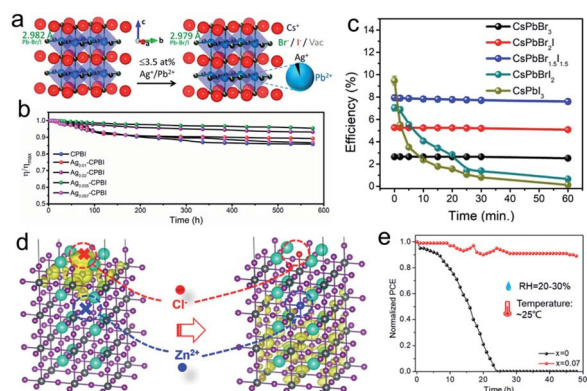
Fig. 16 Compositional engineering for stability. (a) Schematic representation of pristine and Ag-doped CsPbBr 3 crystal structures. Vac indicates anion vacancy. (b) Stability plots for the devices monitored for 575 h (24 days) under an ambient environment. Adapted with permission from ref. 65 Copyright 2021, American Chemical Society. (c) PCE for different compositions of CsPbBr 3-x I x QDs. Adapted with permission from ref. 70 Copyright 2020, Science Direct. (d) Electronic charge density for the pristine CsPbI 3 and CsPb 1-x Zn x I 3 slab with lead and iodide vacancy defects. (e) Ambient storage stability of the SCs without encapsulation. Adapted with permission from ref. 63 Copyright 2020, American Chemical Society.
