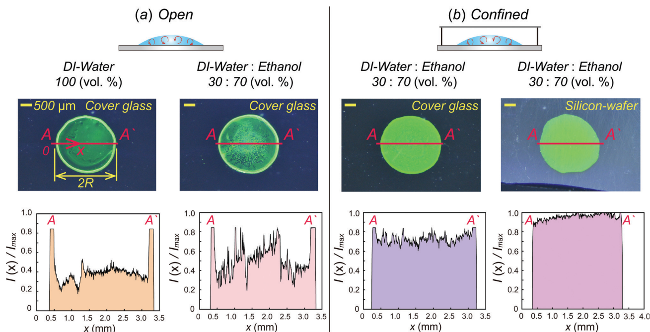
Fig. 5 Comparison of water-soluble QDs deposition patterns with different conditions; (a) open and (b) confined space. (a) Image of water-soluble QD deposition patterns on a cover glass and corresponding intensity profiles I(x) normalized with I_{\max} for pure DI-water and binary mixture (ethanol : DI-water = 70 : 30 vol%) on open substrates. (b) Water-soluble QD deposition patterns and corresponding intensity profiles I(x) normalized with I_{\max} for binary mixture (ethanol : DI-water = 70 : 30 vol%) deposited on a cover glass and silicon-wafer, respectively, in the confined geometry. Solutions are prepared as DI-water : QDs = 99.9 : 0.1 wt% for pure DI-water and ethanol : DI-water : QDs = 44.1 : 55.7 : 0.2 wt% for the binary mixture.
