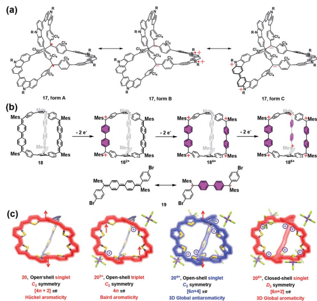
Fig. 8 (a) Three dimensionally \pi -conjugated diradicaloid molecular cage 17 and its three typical resonance forms. Reproduced from ref. 30. (b) Chichibabin's hydrocarbon (CH) based radicaloid cage 18 and its three oxidation states ( 18^{2+} , 18^{4+} and 18^{6+} ), followed by the resonance of CH analogue 19 on the bottom. Reproduced from ref. 31. (c) Three-fold symmetrical diradicaloid cage 20, its three oxidation states ( 20^{2+} , 20^{4+} and 20^{6+} ), the corresponding \pi -electron delocalization pathways and the applied aromaticity rules. Reproduced from ref. 32.
