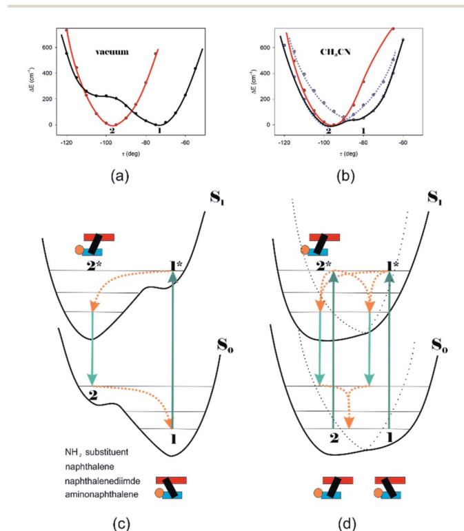
Fig. 6 The (TD)-CAM-B3LYP/D3/TZV calculated S 0 (black) and S 1 (red) state potential energy profiles against the naphthalene twist \tau angle for (a) NDI-BINAM in a vacuum also representing CCl 4 , CH 2 Cl 2 , CHCl 3 , CS 2 , C 6 H 12 , DMSO, and pinene solutions, and (b) CH 3 CN@(NDI-BINAM) also representing CH 3 NO 2 and C 6 H 5 CN solutions where different Sol@(NDI-BINAM) produces profile asymmetry (grey and violet dotted branches). ca. 40 kcal mol -1 downshift of the S 1 potentials is to highlight the differences. (c) and (d) the S 0 and excited S 1 asymmetric potential profiles illustrating the genesis of the RROA and ECD sign concordance, and (d) bisignate RROA: dotted branches denote the presence of different Sol@(NDI-BINAM) positions. Green and orange denote radiative and radiationless processes, respectively.
